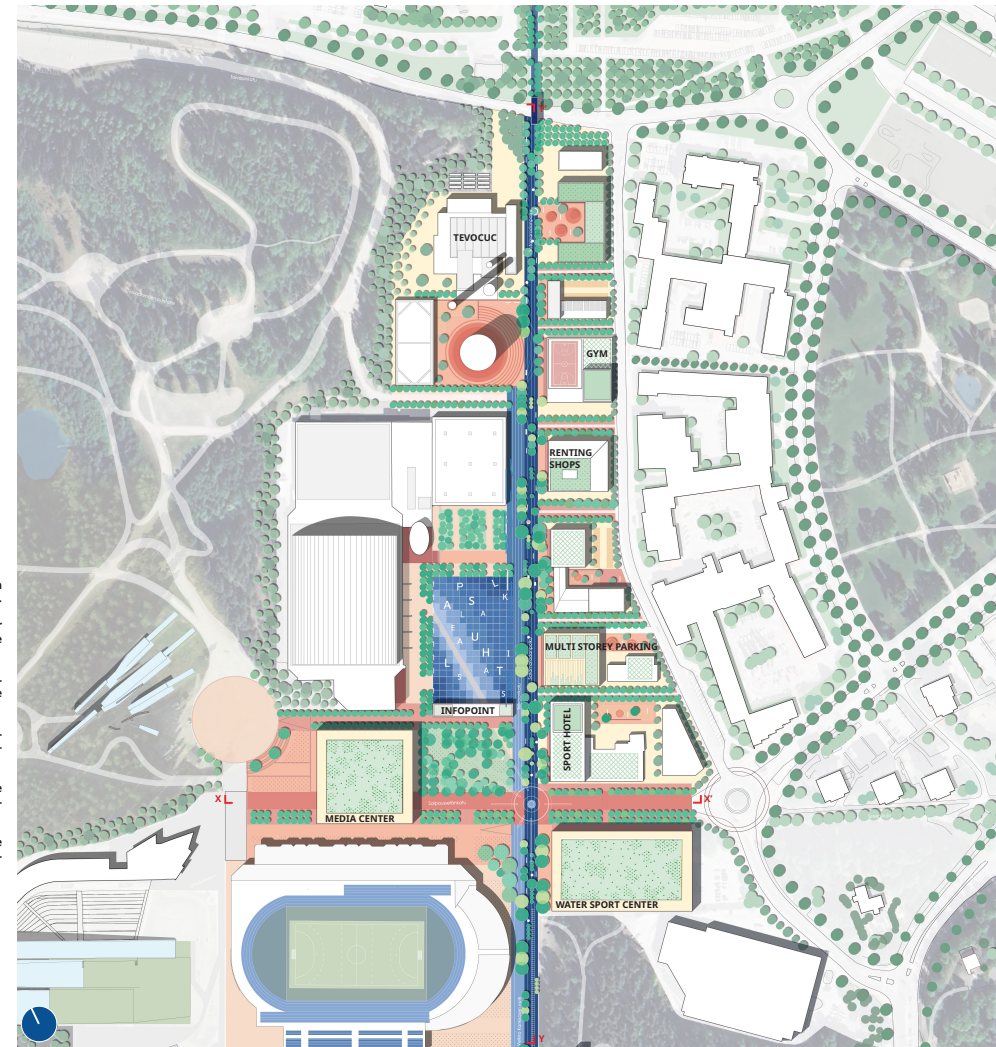
1.2000 Masterplan
