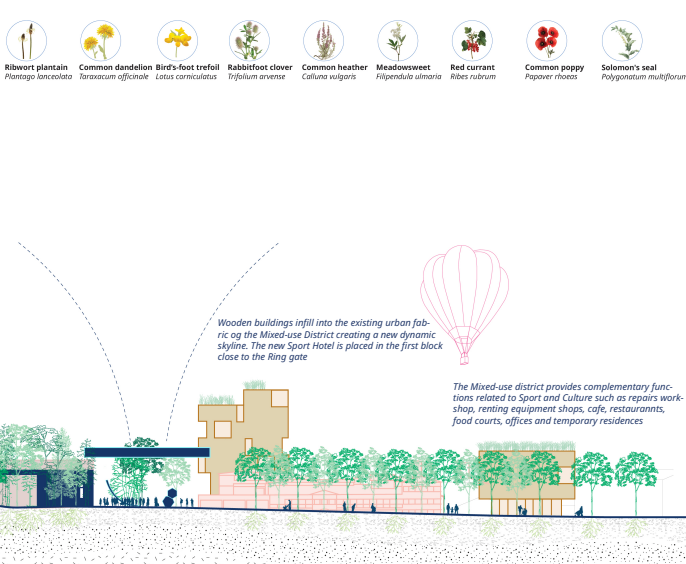
1.800 Section X-X' Central area along Salpausselkäkatu Street
